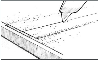
Figure 26 Trim overlapped cloth after the epoxy gels.
