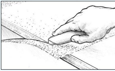
Figure 25 Trim excess cloth after the epoxy gels but before it cures hard.
